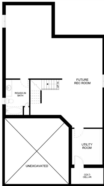
FOUNDATION PLAN
